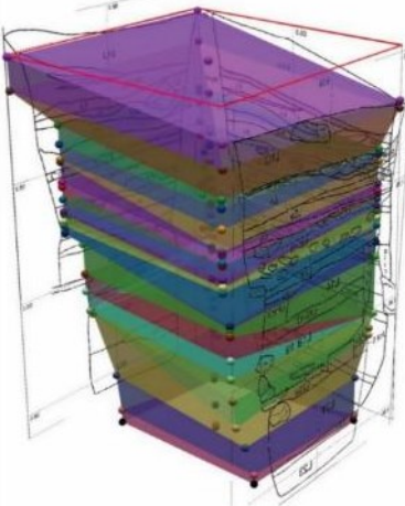
Figure 6 Cave topography and location of trenches within East Chamber (Survey by T. Chadzitheodorou, EPSNE).
