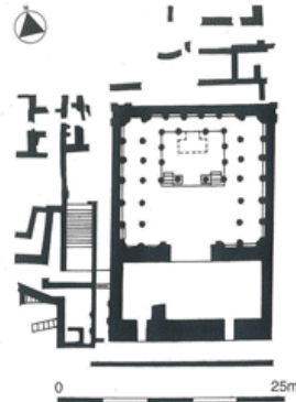
245. Plan of the Temple and its annexes. In a fashion typical of a Nabataean sanctuary, its ground plan consists of a shallow portico, a square cella, and a central platform altar, or mdtob .
